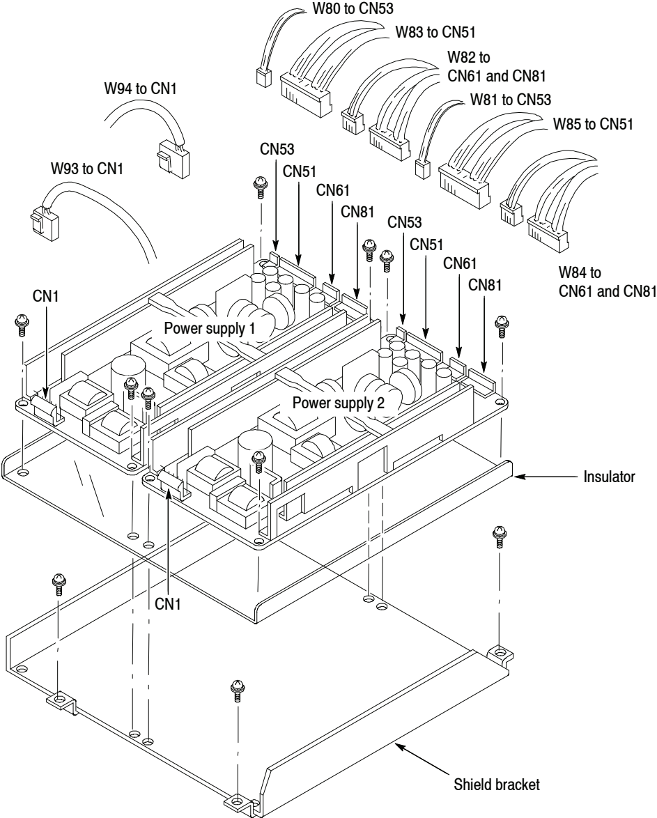
Figure 5-24: Power supply 1 and 2 removal
