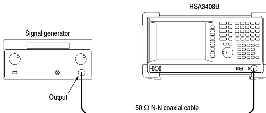
Figure 4- 11: Test hookup
