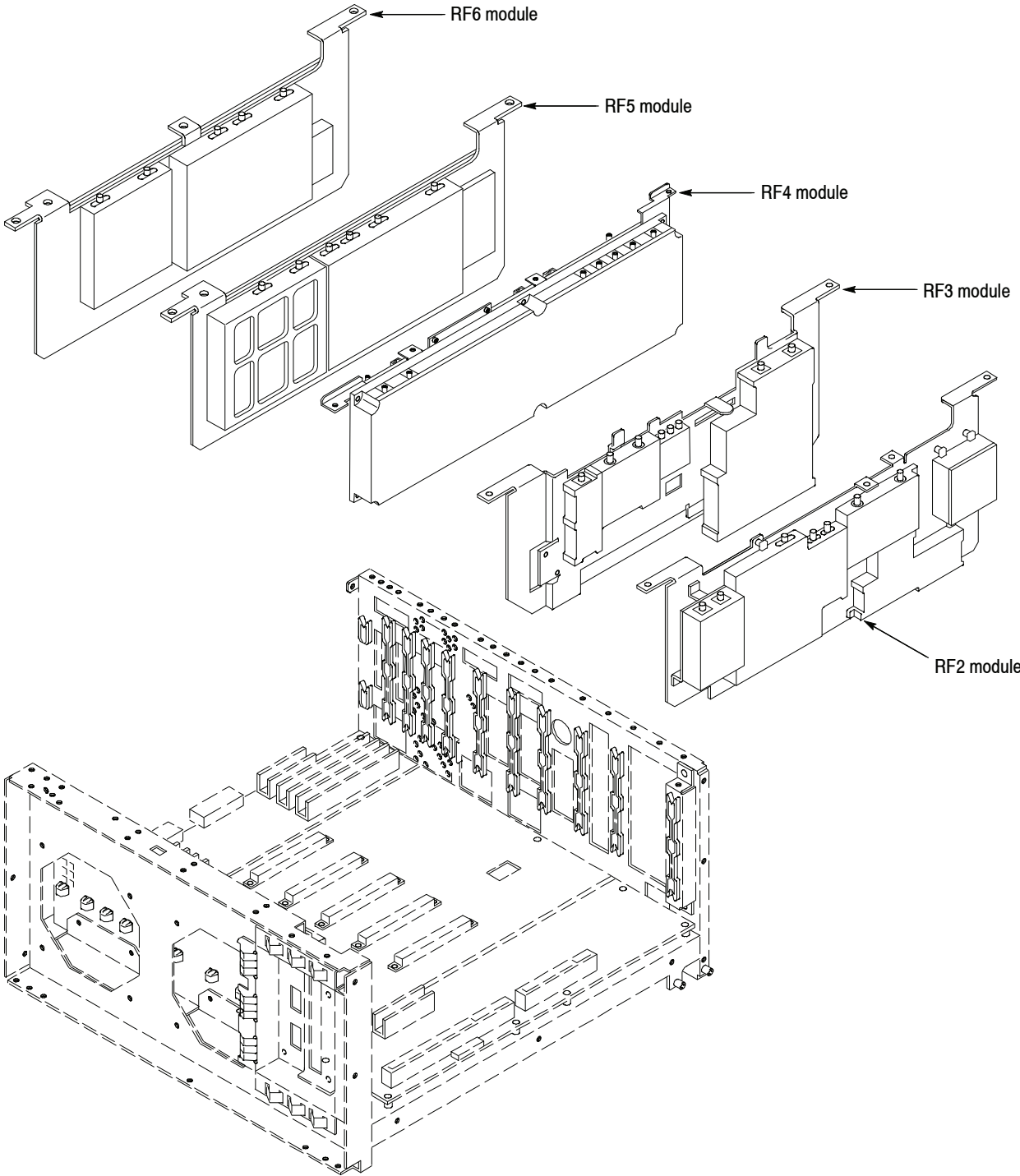
Figure 5-3: RF modules
